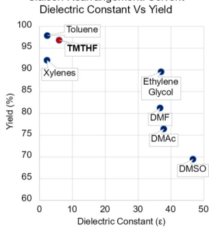
Chart 1: Effect of solvent dielectric constant on reaction performance.
